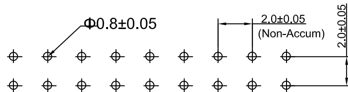
PCB Layout
