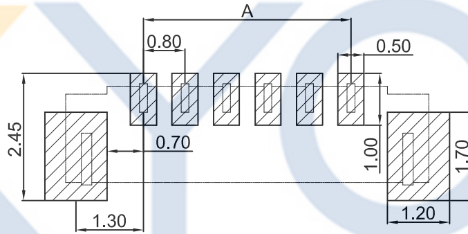
PCB LAYOUT
