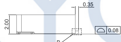
DETAIL B SCALE 1:1
