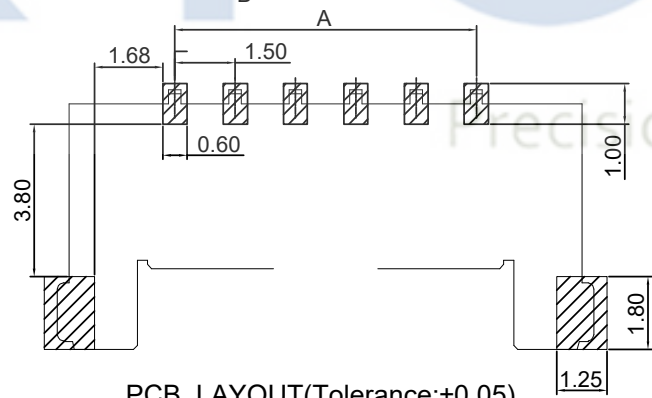
PCB LAYOUT(Tolerance:±0.05)
