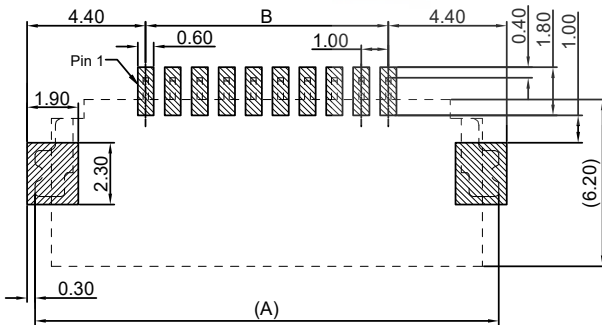
RECOMMENDED PCB PATTERN DIM. TOLERANCE:±0.05
