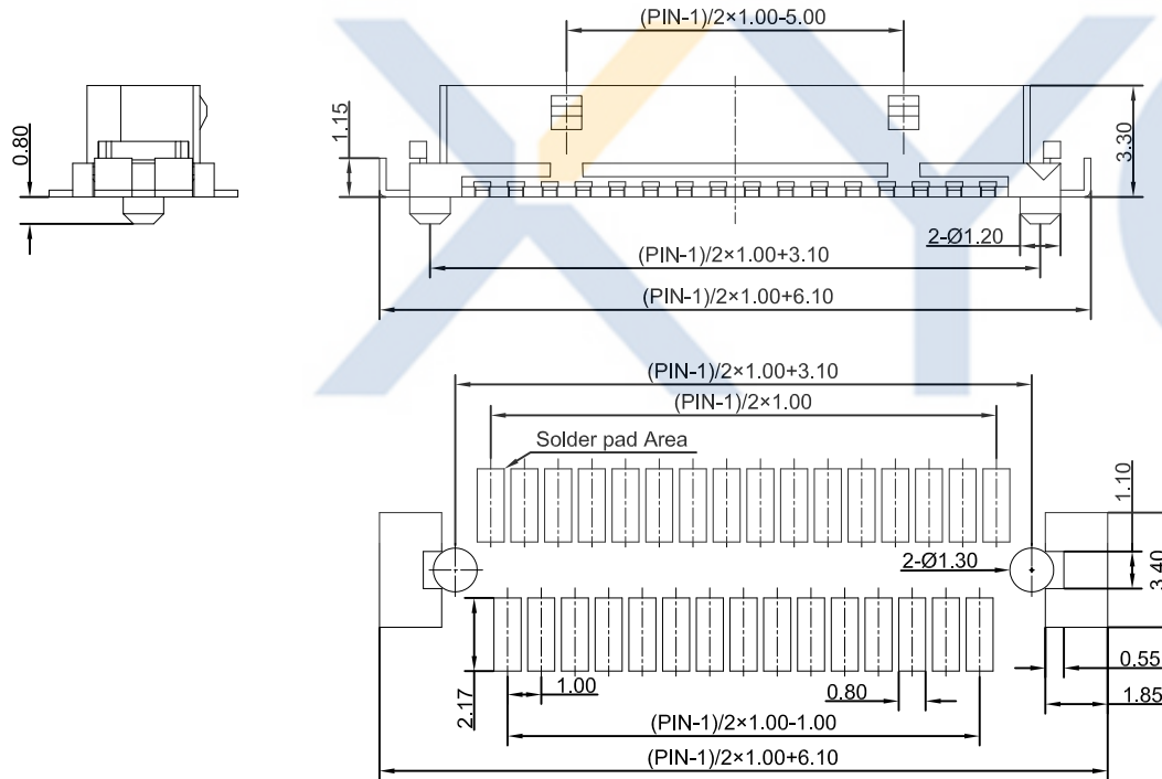
Recommended P.C.B Layout(Top Side)
