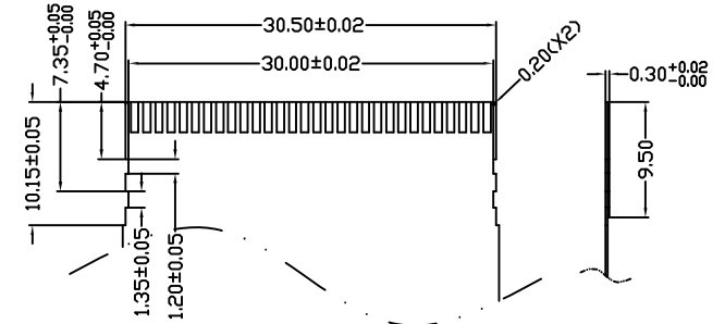
FFC WIRE
